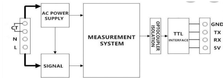
Fig. 4. The block diagram of pzen-004t
