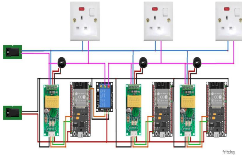
Fig. 1. The Proposed wireless smart metering system design.
