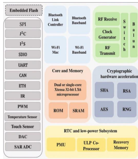
Fig. 3. The block diagram of ESP32.
