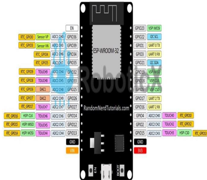
Fig. 2. The ESP32 Microcontroller
