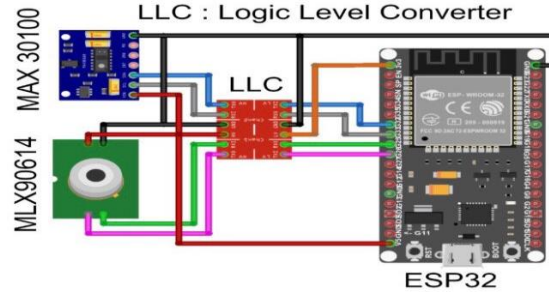
Fig. 6. The circuit connection between the sensors and microcontroller
