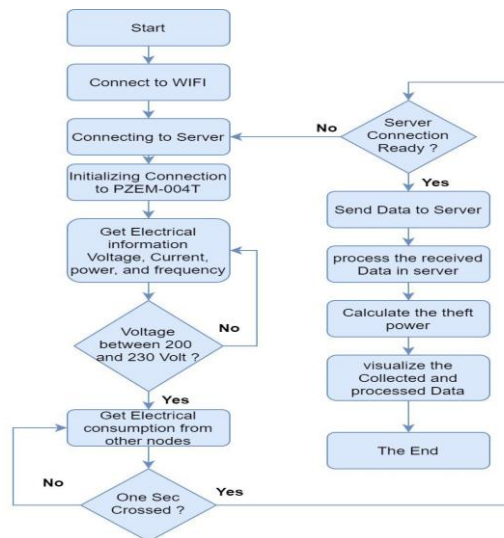
Fig. 5. The flowchart of an electrical energy management system based on IoT
