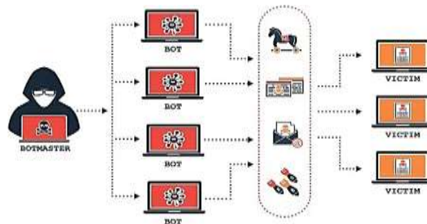
Figure 11: Botnets Attack
